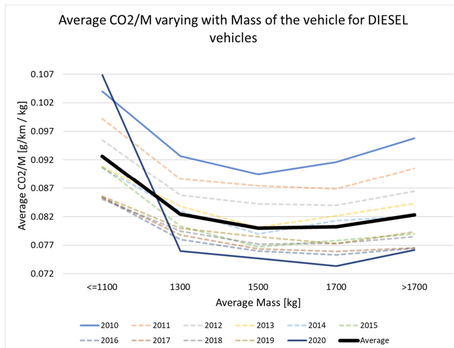
Figure 11: Average CO 2 /M of diesel vehicles for mass categories per year. Diesel vehicles below 1100 kg is a very minor group, and the 2020 data for this group is of little relevance.
