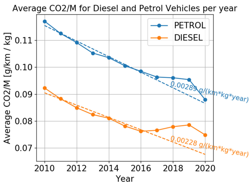
Figure 17: Yearly fleet average of \text{CO}_2/\text{M} in \text{g}/(\text{km} \cdot \text{kg}) in the EU for petrol and diesel vehicles.
